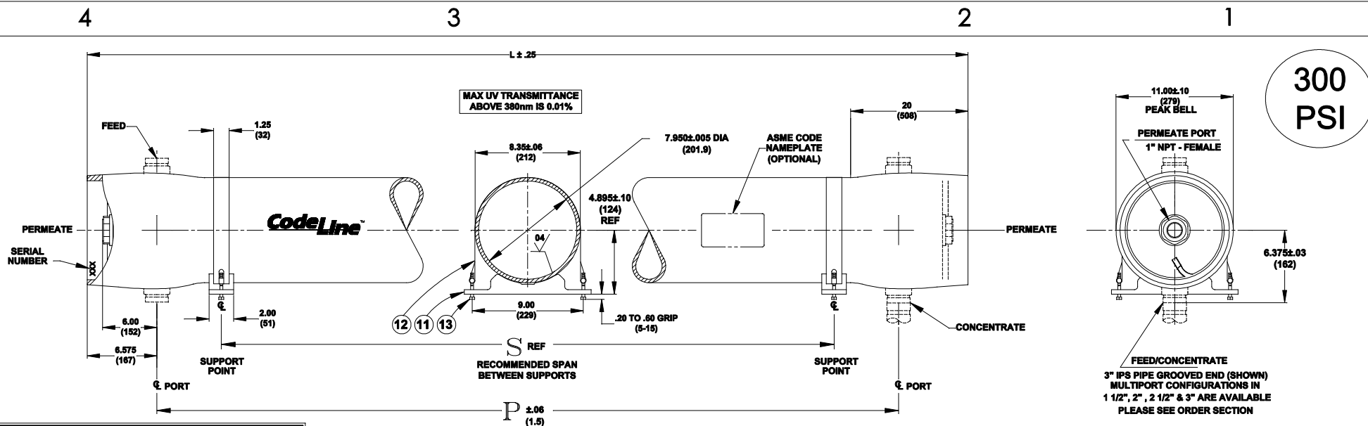
VIEW AT CENTER SUPPORT CENTER VESSEL ON 2 OR 3 SUPPORTS AT SPAN(S) "S" : 3 SUPPORTS REQUIRED
